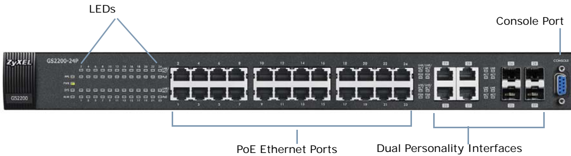
Figure 12 Front Panel (GS2200-24P)
