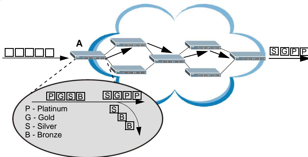
Figure 154 DiffServ Network
